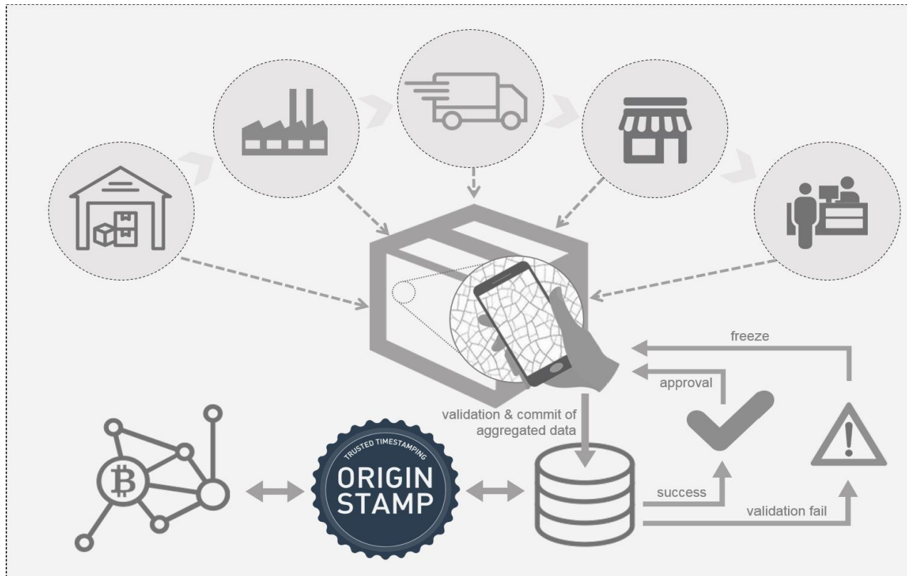
Figure 2: The figure illustrates the process of tracking a physical asset with a mobile phone camera. Each time the craquelure is scanned and verified, the corresponding meta-data, i.e. perceptual hash, location, or temperature, is encrypted, hashed, appended and finally timestamped with Origin Stamp.
