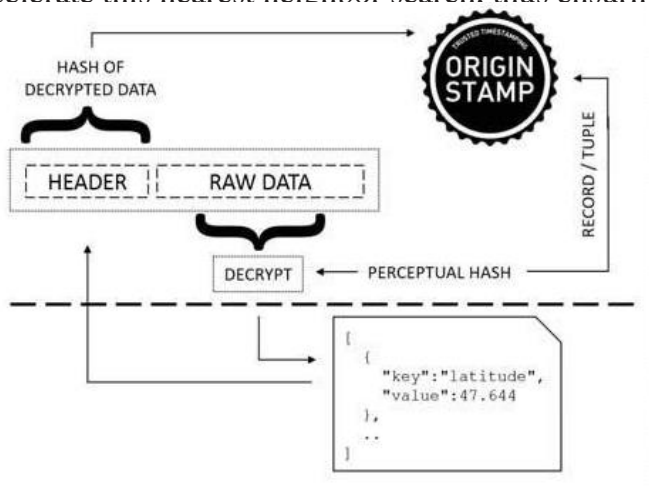
Figure 3: The encrypted data-structure in HEX format that is stored on the server and timestamped with Origin Stamp consists of mainly two parts: Header and Raw Data.
